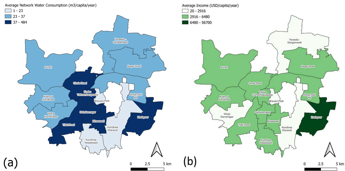
Figure 7. (a) Spatial distribution of average network water consumption (m 3 /capita/year) (Zhu, in preparation) in Pune, India, by administrative wards. (b) Spatial distribution of income (USD/capita/year) (Zhu, in preparation) in Pune, India, by administrative wards.
